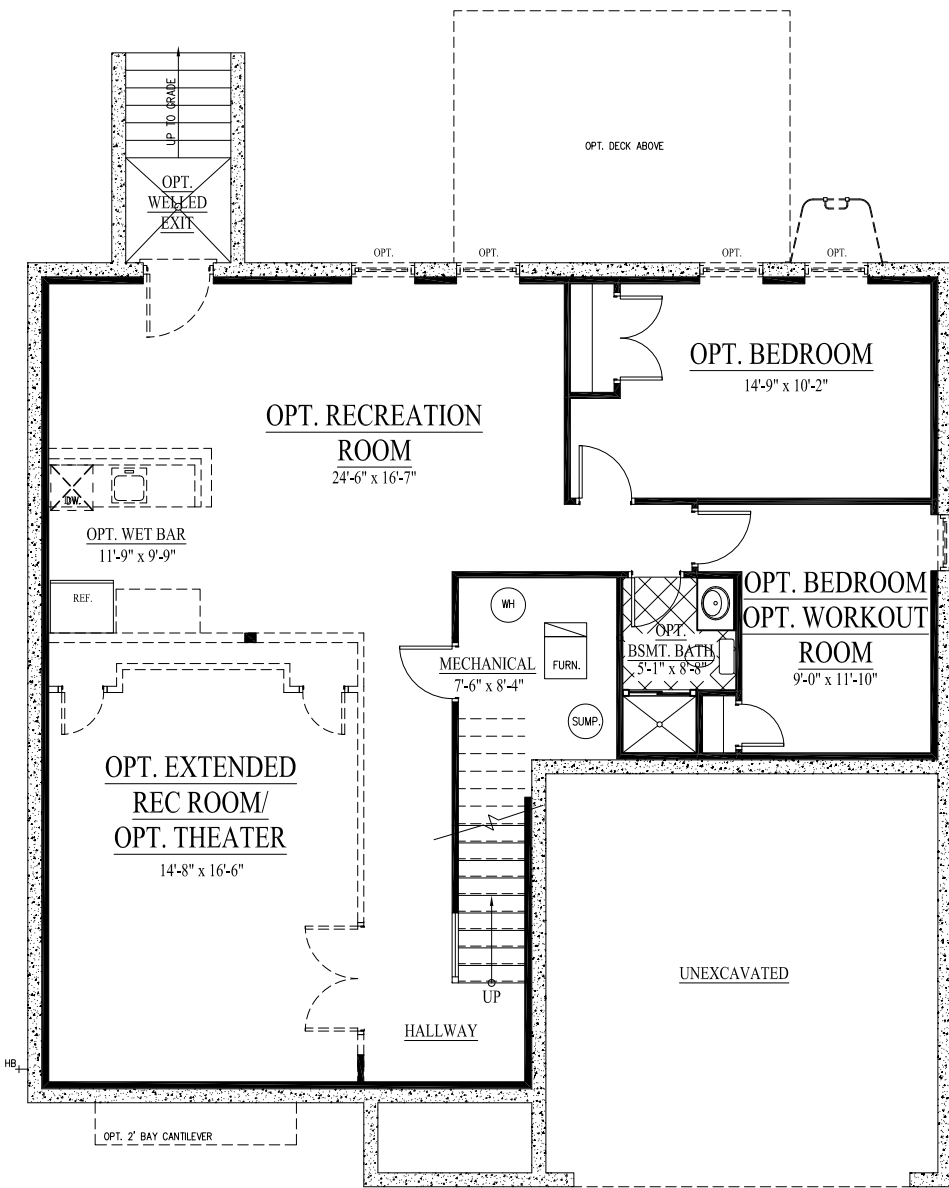
BASEMENT FLOORPLAN
