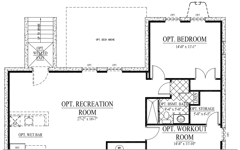
BASEMENT W/ OPT. SUNROOM
