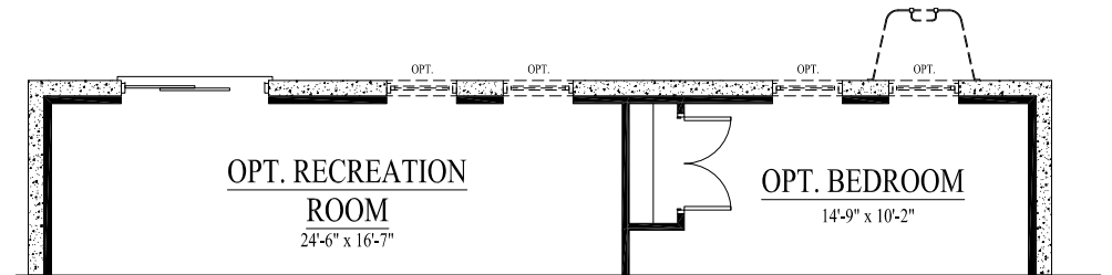
BASEMENT W/ OPT. WALKOUT
