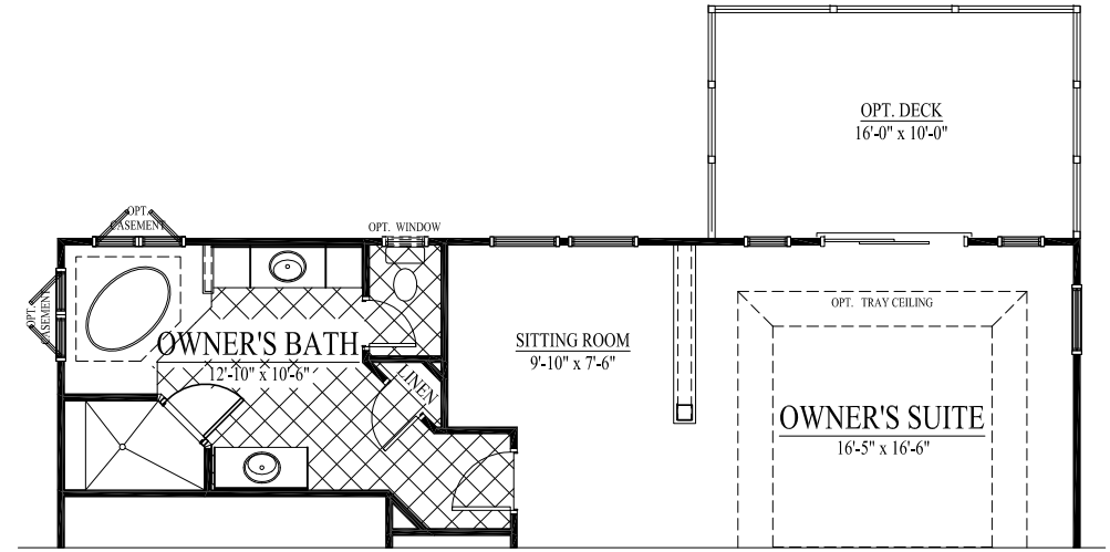
SECOND FLOOR W/ OPT. VIEWING DECK
