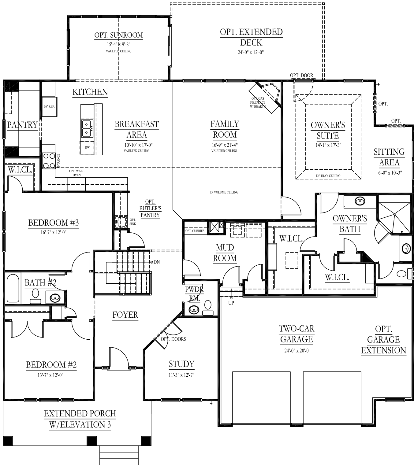
MAIN LEVEL FLOOR PLAN W/ OPT. SUNROOM, OPT. GARAGE EXTENSION, OPT. BUTLER'S PANTRY AND ELEVATION 3 PORCH
