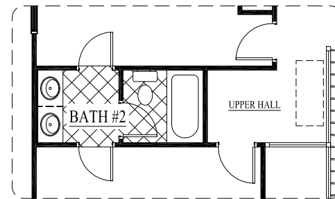
OPT. BUDDY 2ND BATH
