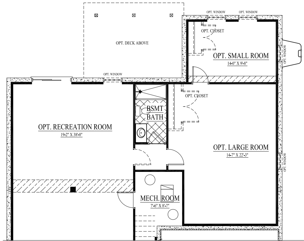
SUNROOM OPTION W/OPT. WALKOUT
